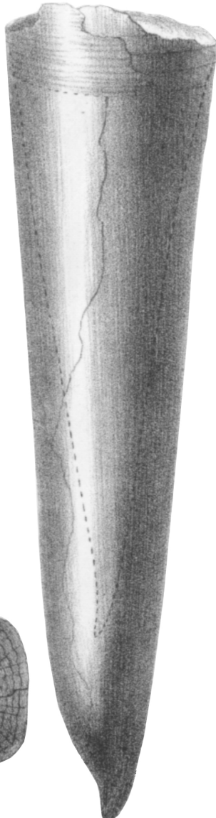
BELEMNITES.
